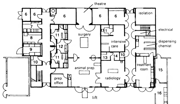
5 Ground floor of → 4
